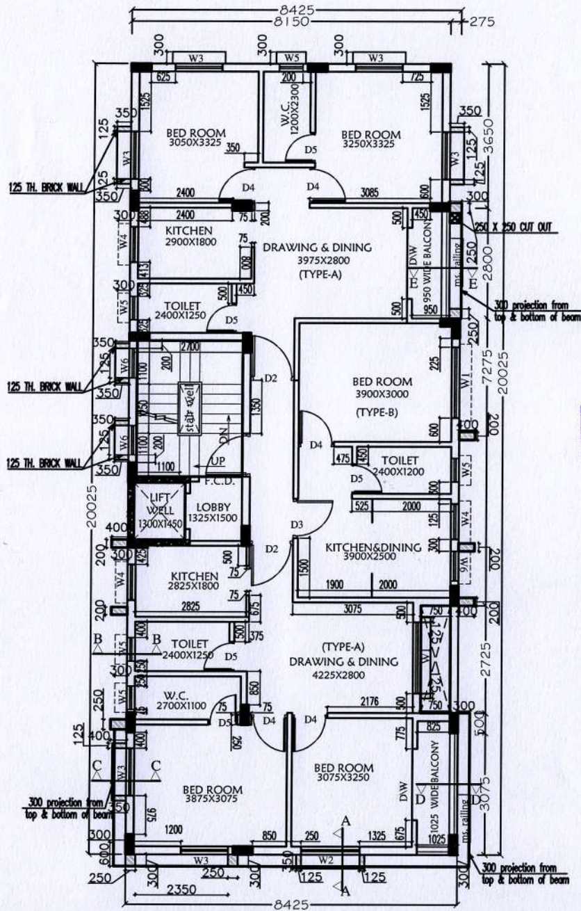
THIRD FLOOR PLAN SCALE :- 1:100
